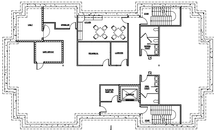
BASEMENT FLOOR PLAN 1/8" = 1'-0"
