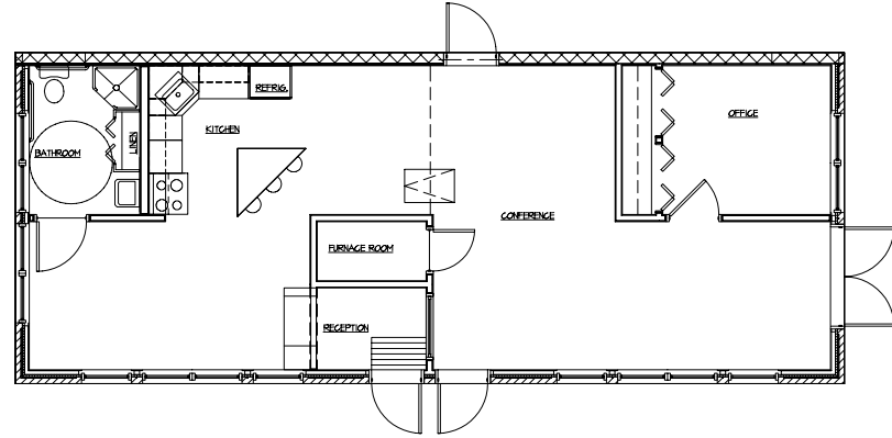
NEW OFFICE FLOOR PLAN SCALE: 1/4"=1'-0"
