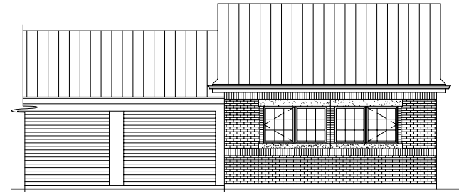
PARTIAL NORTH ELEVATION SCALE: 1/4"=1'-0"
